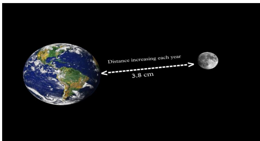
Figure.1 Moon's distance increasing each year
