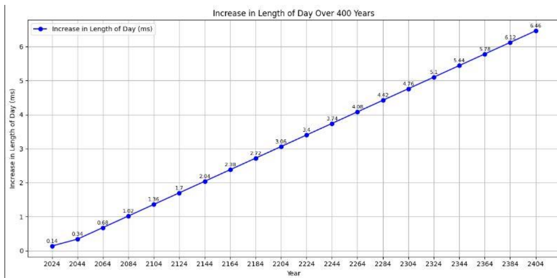
Figure. 3: Projected Increase in Length of Day (ms) from 2024 to 2404
