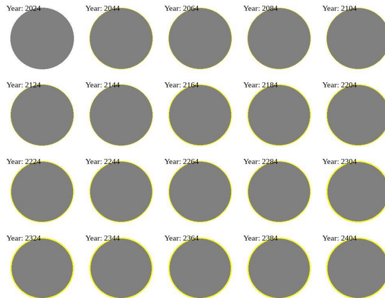
Figure 6: "Evolution of the Moon's Angular Diameter During Solar Eclipses (2024-2404)"
