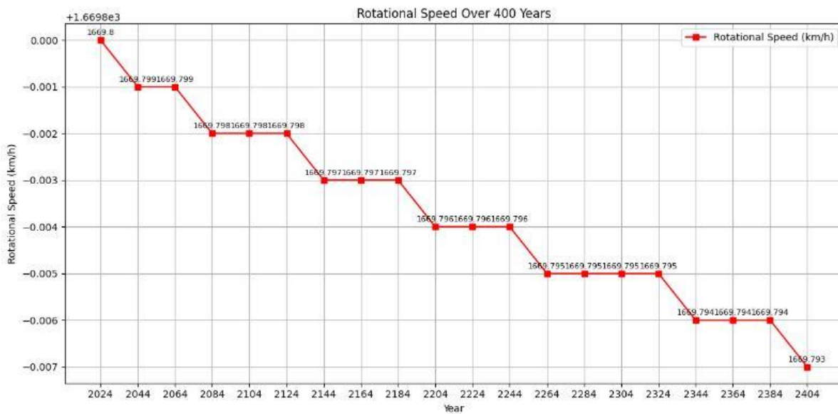
Figure. 4: Projected Decrease in Earth's Rotational Speed (km/h) from 2024 to 2404
