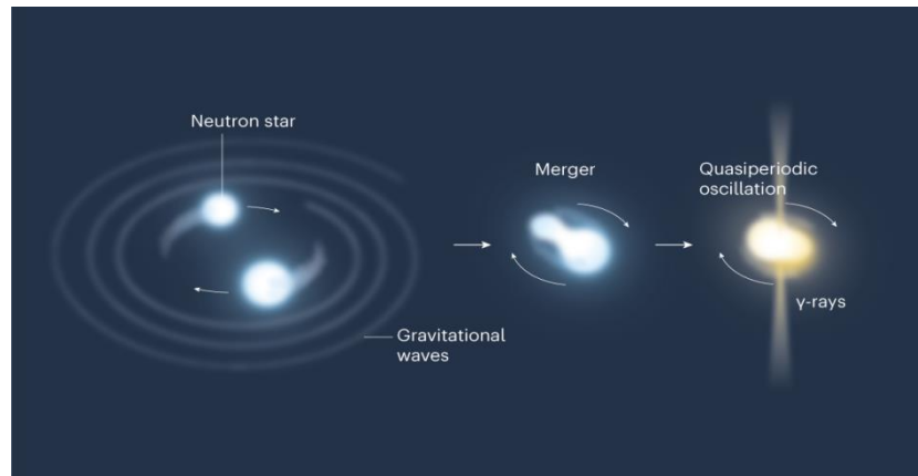
Fig.5 Gravitational waves produced by Neutron star collision
