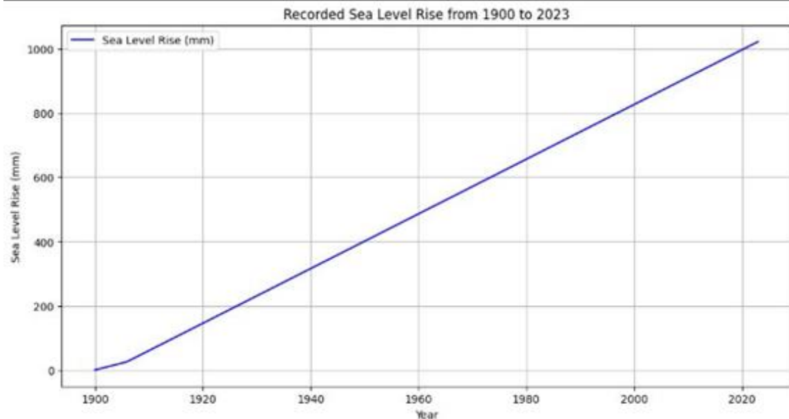
Figure-2 Data of sea level risen from 1900 to 2023 year
