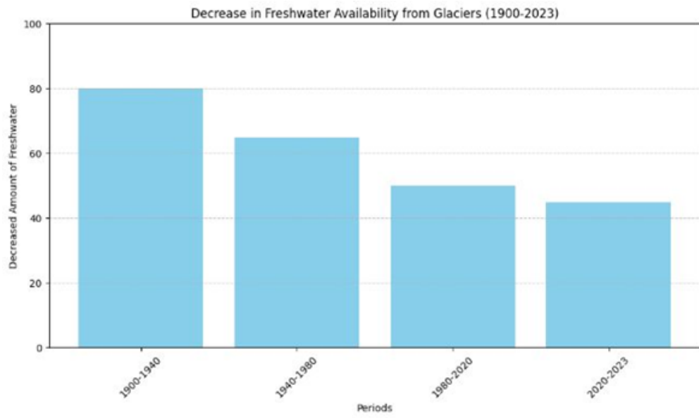
Figure-3 Decrease in Freshwater Availability from Glaciers (1900-2023)
