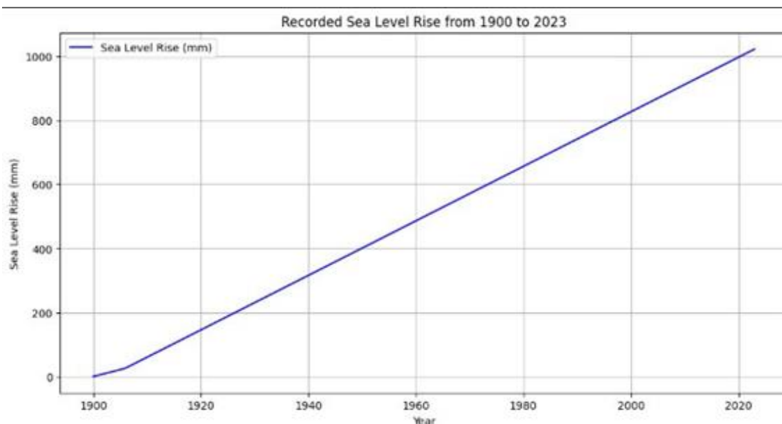
Figure-2 Data of sea level risen from 1900 to 2023 year
